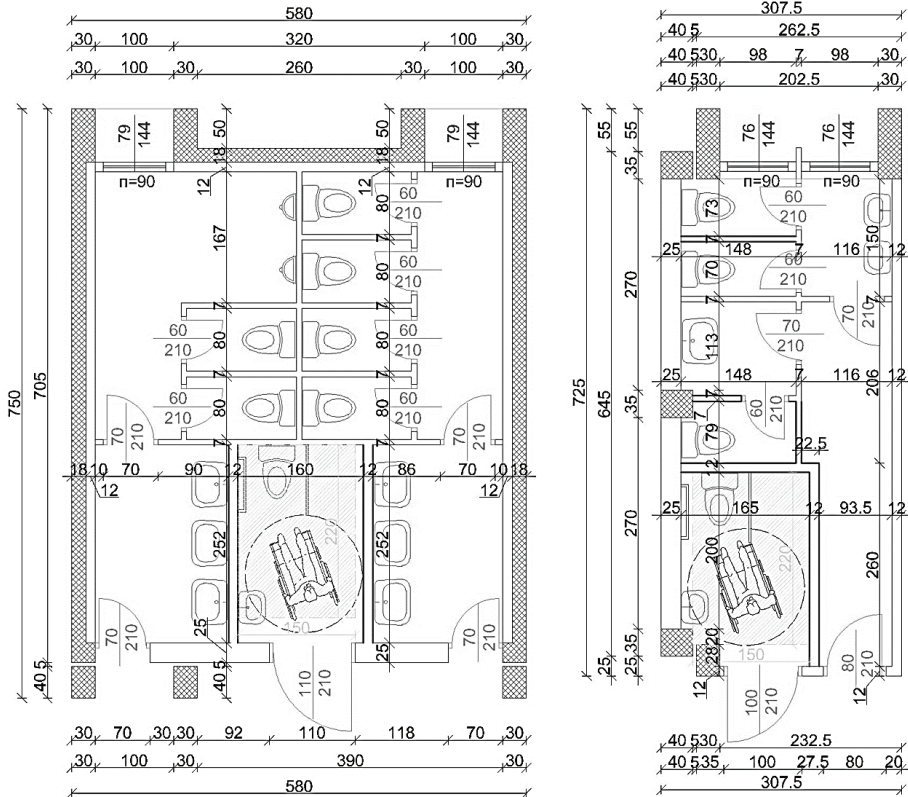
Adaptations to provide an independent sanitary unit for people with disabilities
